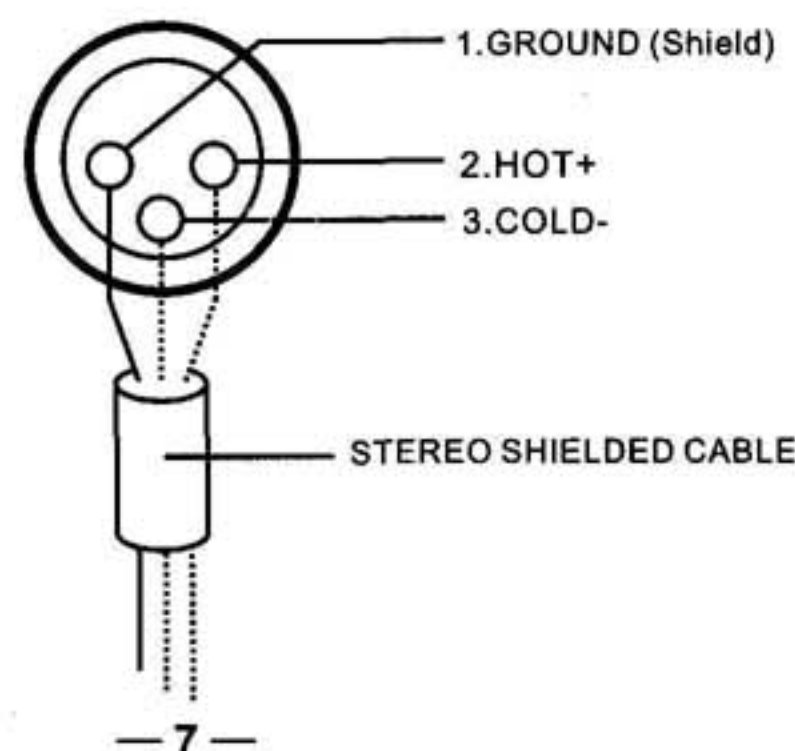
FEMALE 3 PIN CONNECTOR
