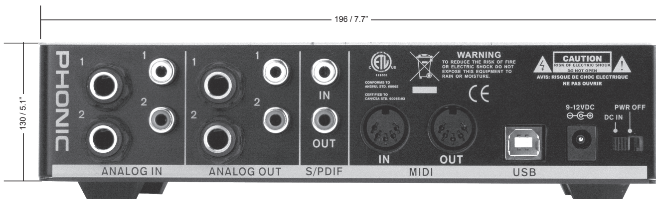
Back Panel
